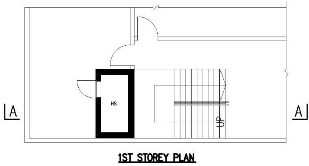
FIGURE 2.4.1c (i) RC/CLAY TILED ROOF COVER OVER STAIRCASE NEAR HS WALL IN A LANDED DEVELOPMENT
