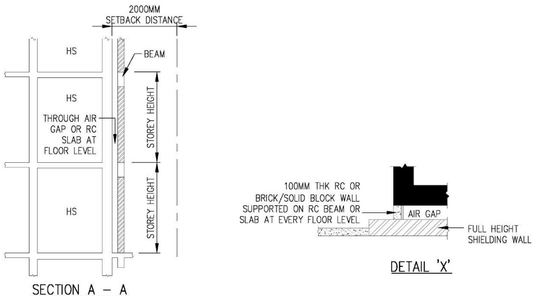
FIGURE 2.4.5(d) SHIELDING WALL “A” AND “B” FOR HS WITH SHORTEALL OF SETBACK DISTANCE ON TWO SIDES OF HS (TYPE 2A)
