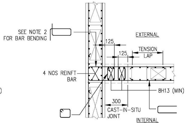
PRECAST CONNECTION DETAIL ABOVE STARTER REINFORCEMENT BAR LEVEL (TYPE 2)
