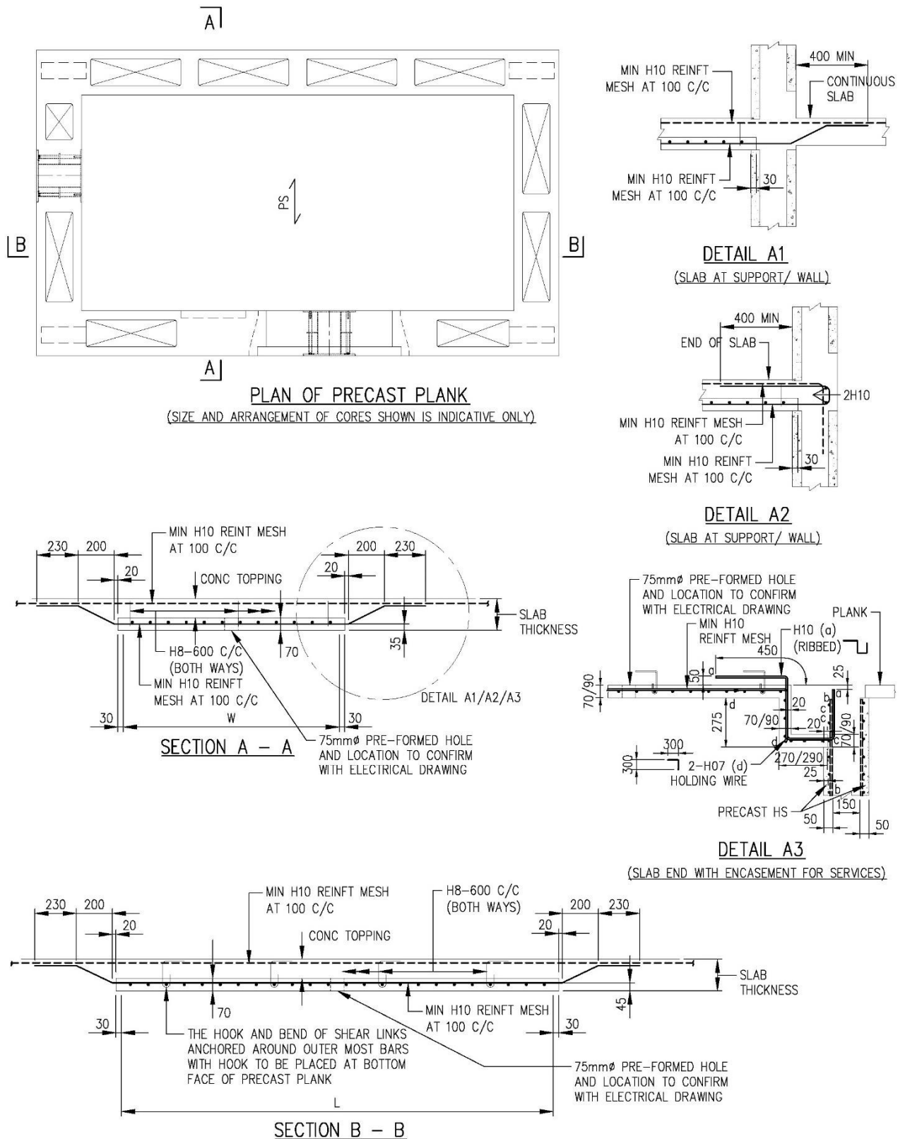
FIGURE 3.5.6.3(i) DETAILS OF PRECAST PLANK (MARKED AS PS) AND CONCRETE TOPPING
