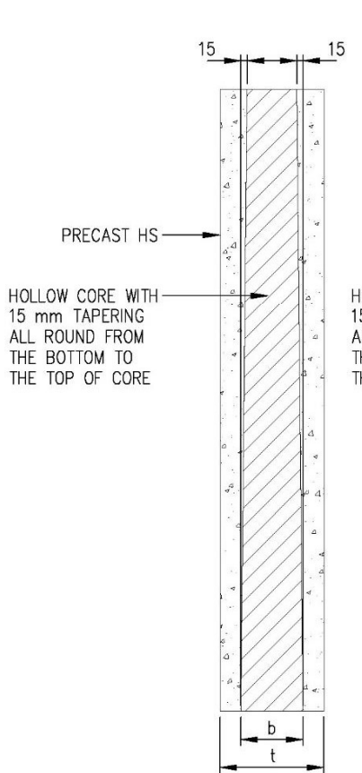
SECTION 1 - 1
