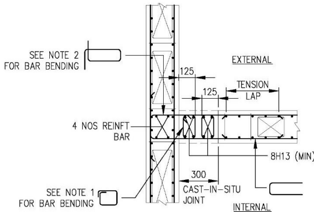
PRECAST CONNECTION DETAIL AT STARTER REINFORCEMENT BAR LEVEL (TYPE 2)
