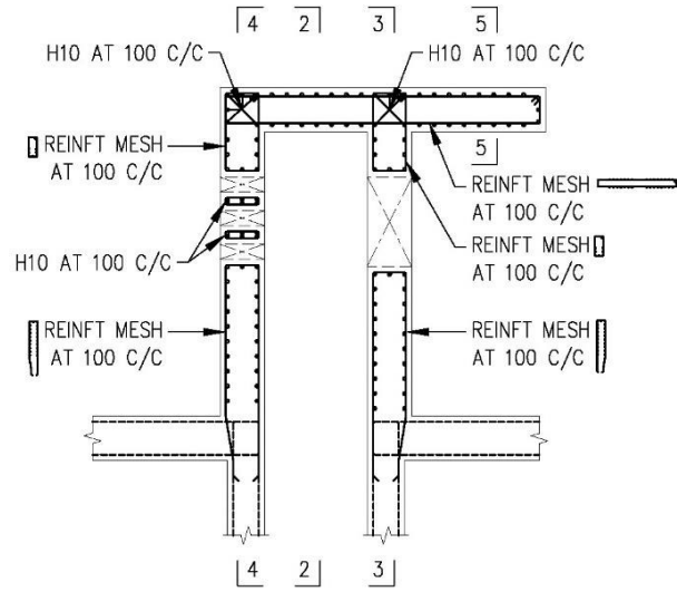
SECTION 1-1
