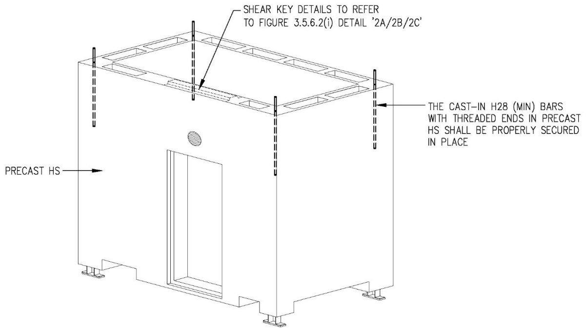
ISOMETRIC VIEW FROM TOP (TYPE 1)
