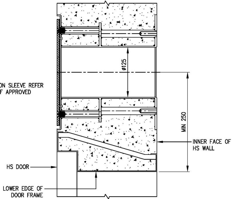
VENTILATION SLEEVE AT CLOSED POSITION
