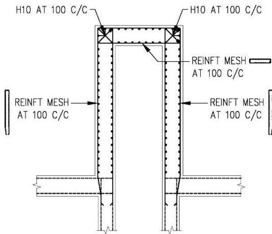
SECTION 2-2
