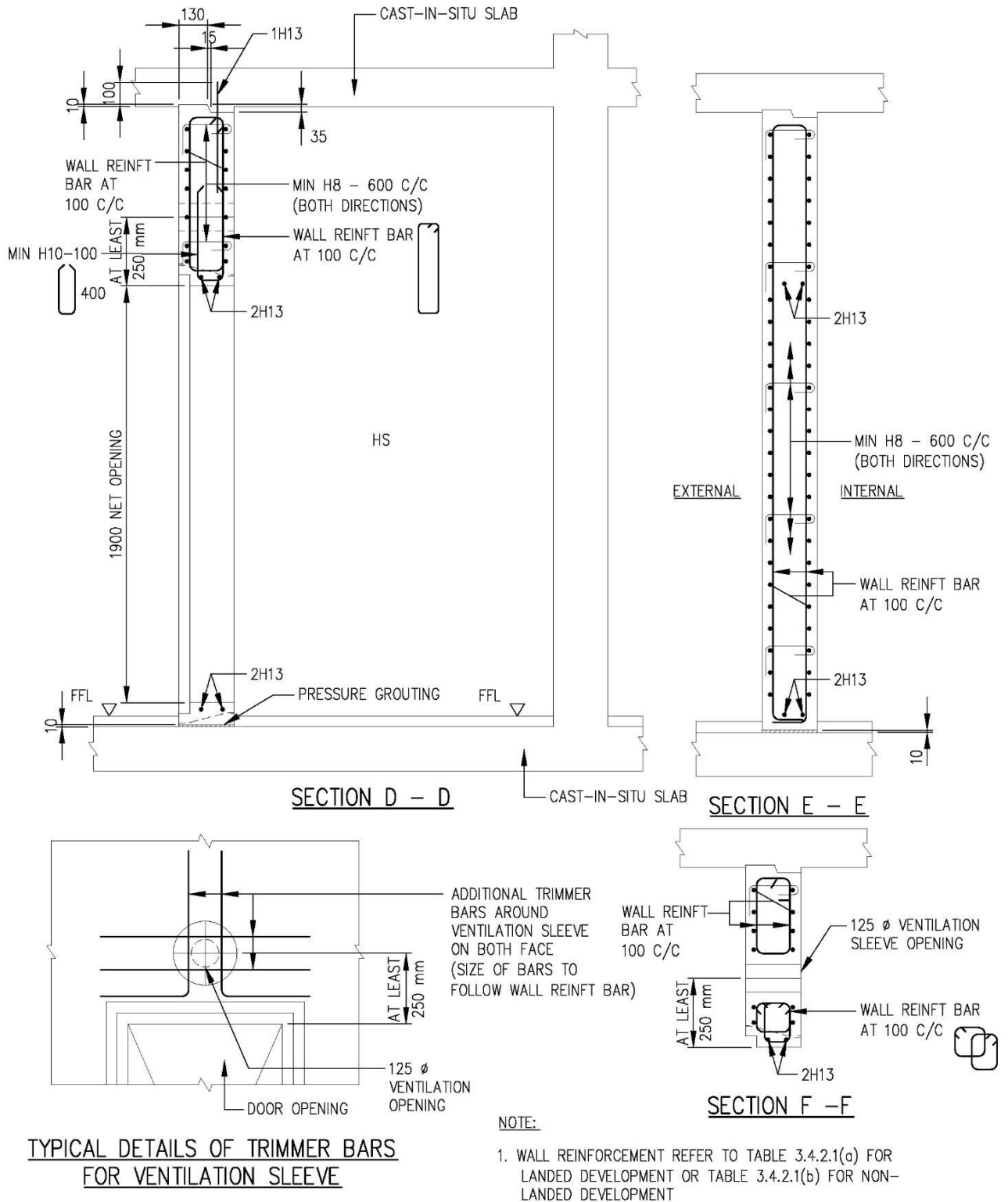
FIGURE 3.5.5(h) SECTIONS OF PRE-CAST HS DOOR FRAME PANEL WITH VENTILATION SLEEVE ABOVE IT (TYPE 2)
