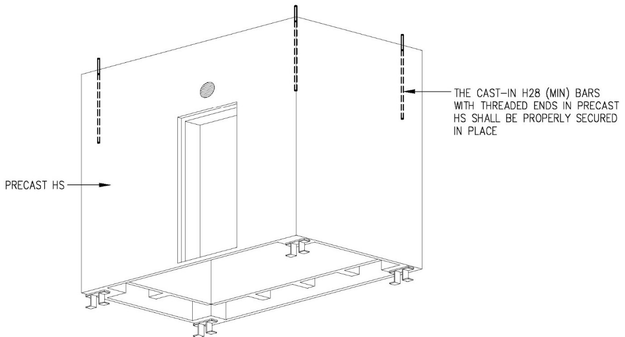
ISOMETRIC VIEW FROM BOTTOM (TYPE 2)
