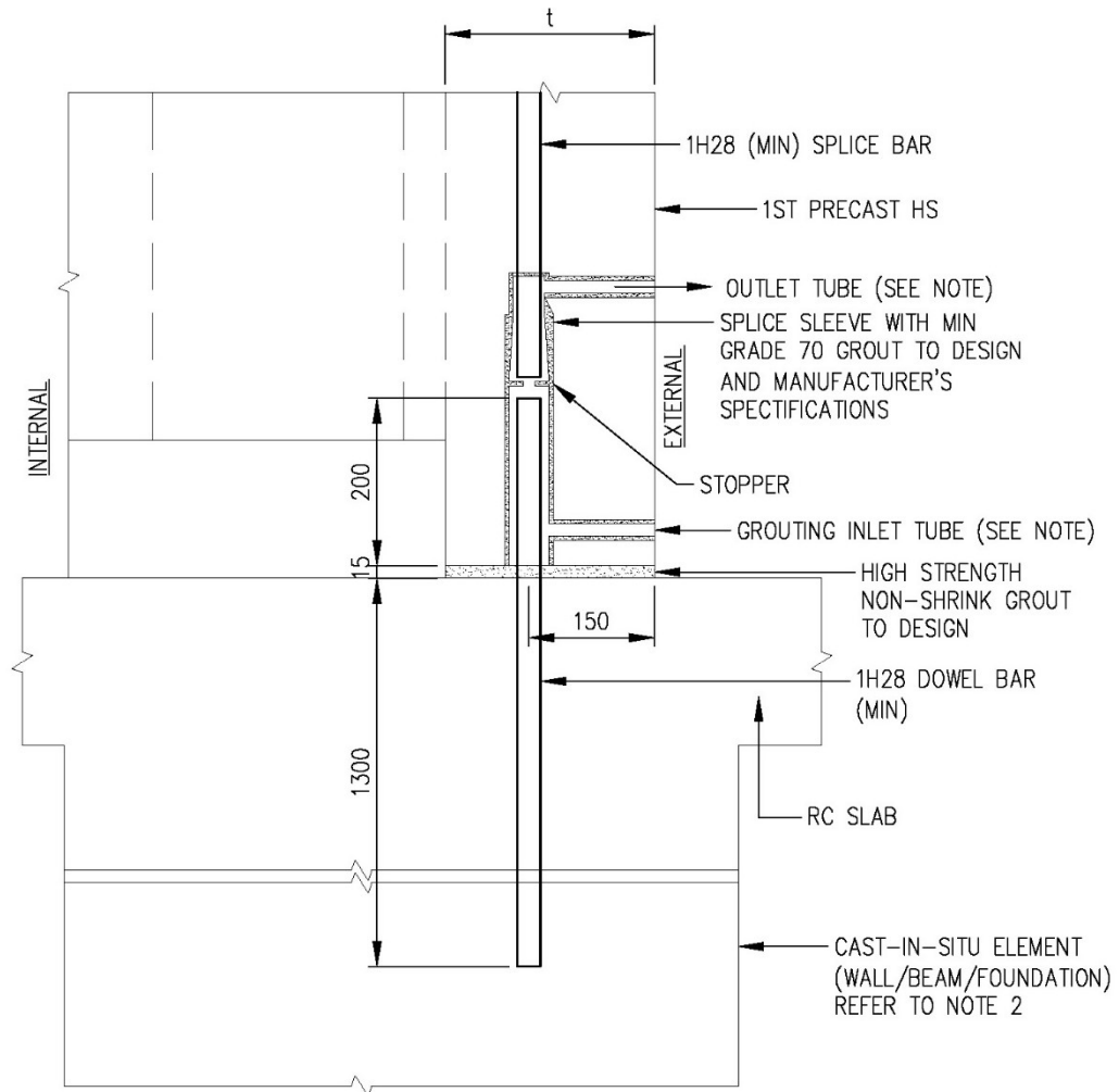
DETAIL 'A' (TYPICAL DETAILS OF H28 (MIN) DOWEL BAR FOR SPLICE SLEEVE CONNECTION BETWEEN 1ST PRECAST HS AND CAST-IN-SITU ELEMENT)
