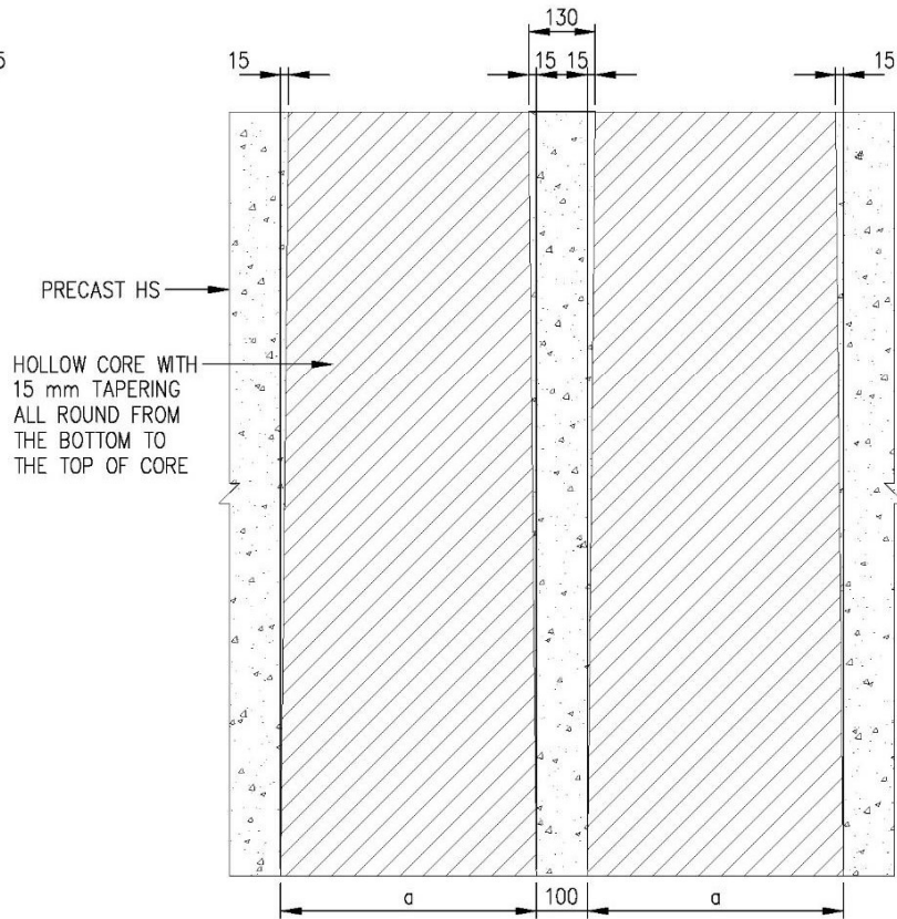
SECTION 2 - 2
