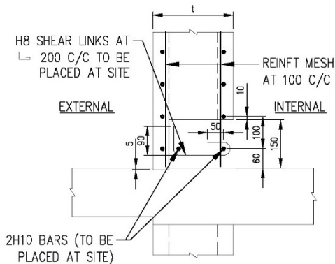
DETAIL '1B' (FOR PRECAST BOTTOM OPENING ON INTERNAL FACE OF WALL)
