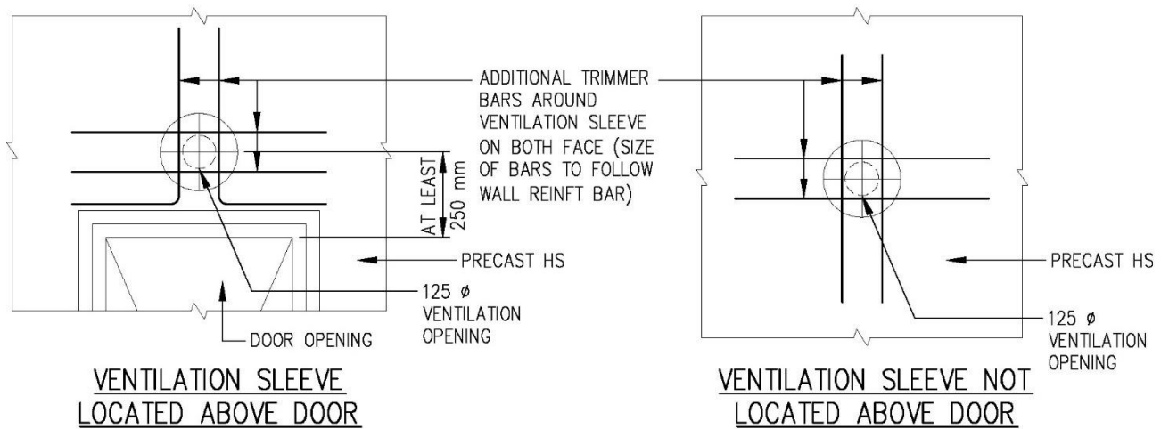
FIGURE 3.5.6.2(j) DETAILS OF TRIMMER BARS FOR VENTILATION SLEEVE
