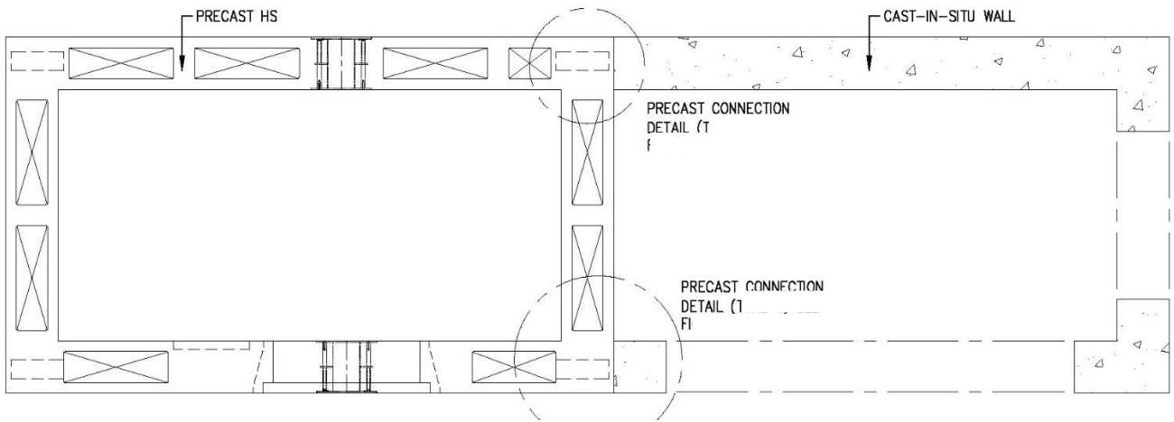
FIGURE 2.6.1(e) PRECAST HS ADJOINING CAST IN-SITU WALLS/COLUMNS
