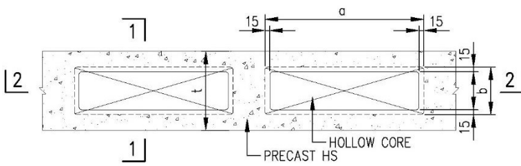
DETAIL 'X'
