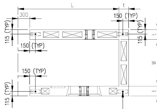
REFERENCE PLAN FOR 1ST PRECAST HS (SIZE AND ARRANGEMENT OF CORES SHOWN IS INDICATIVE ONLY)
