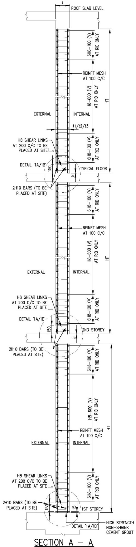
FIGURE 3.5.6.2(h) REINFORCEMENT BAR DETAILS AT CONCRETE RIB
