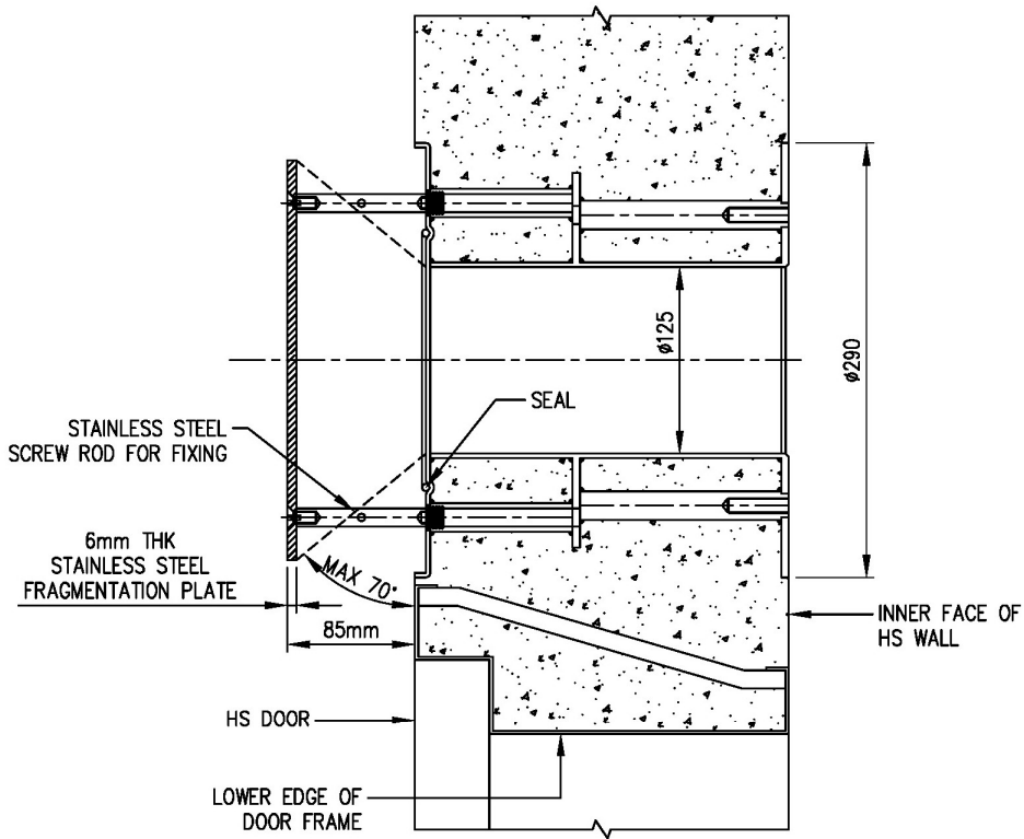
VENTILATION SLEEVE AT OPEN POSITION
