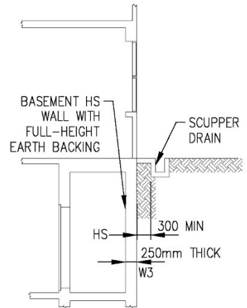
BASEMENT WALL WITH EARTH BACKING AND SCUPPER DRAIN
