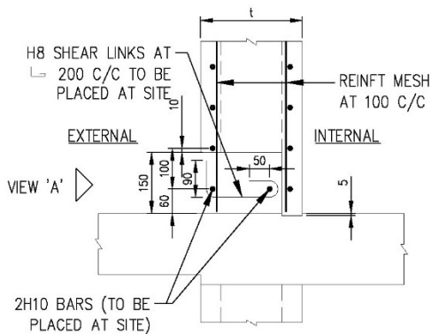
DETAIL '1A' (FOR PRECAST BOTTOM OPENING ON EXTERNAL FACE OF WALL)
