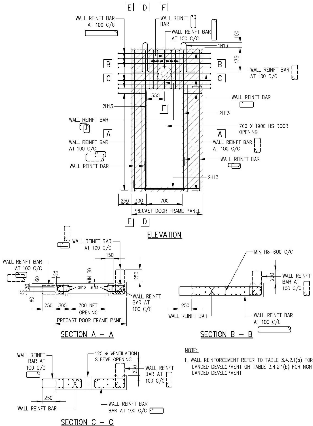
FIGURE 3.5.5(g) DETAILS AND SECTIONS OF PRE-CAST HS DOOR FRAME PANEL WITH VENTILATION SLEEVE ABOVE IT (TYPE 2)
