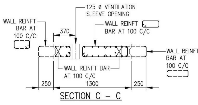
FIGURE 3.5.5(d) DETAILS AND SECTIONS OF PRE-CAST HS DOOR FRAME PANEL WITH VENTILATION SLEEVE AT ITS SIDE (TYPE 1)
