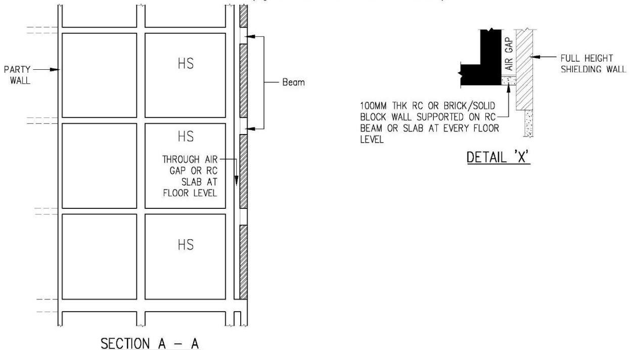
FIGURE 2.4.5(c) SHIELDING WALL “A” AND “B” FOR HS WITH SHORTFALL OF SETBACK DISTANCE ON ONE SIDE OF HS (TYPE 1C)
