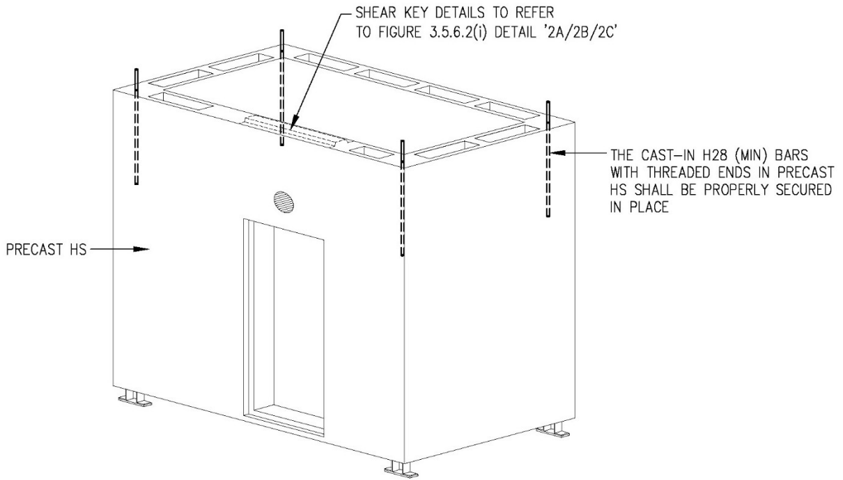
ISOMETRIC VIEW FROM TOP (TYPE 2)
