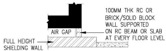
DETAIL 'X'
