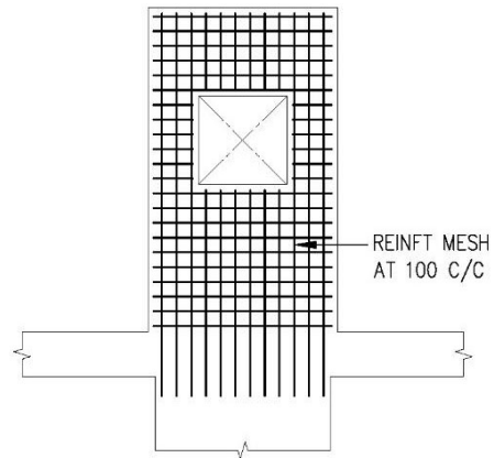
SECTION 3-3
