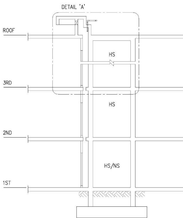
SECTION 1-1
