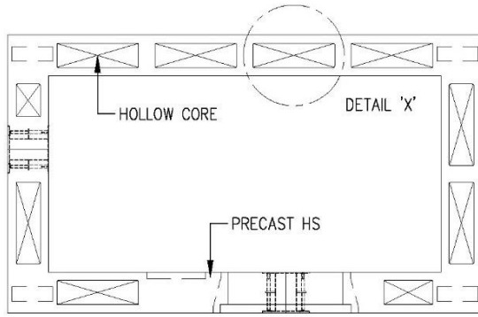
PLAN OF PRECAST HS (SIZE AND ARRANGEMENT OF HOLLOW CORES SHOWN ARE INDICATIVE ONLY)
