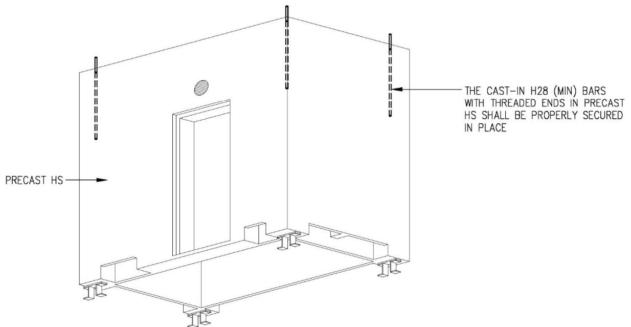
ISOMETRIC VIEW FROM BOTTOM (TYPE 1)
