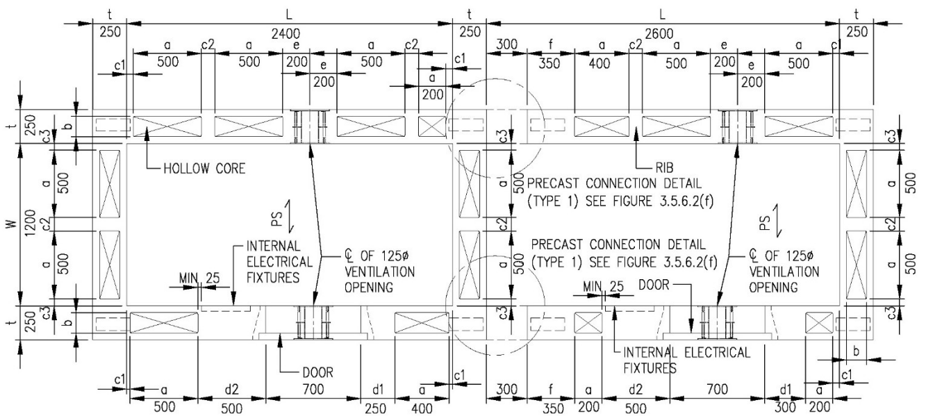
FIGURE 3.5.6.1(c) PRECAST HS SHOWING VENTILATION SLEEVE AND INTERNAL ELECTRICAL FIXTURES ON THE SAME WALL (TYPE 3)
