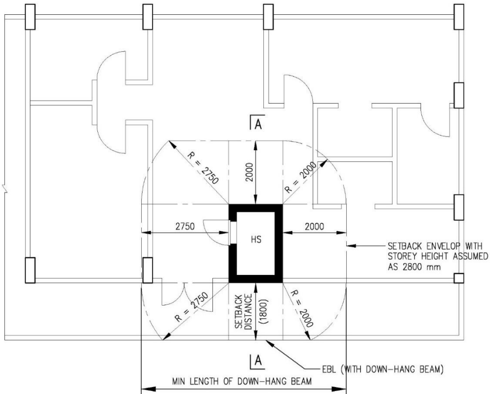
PLAN (E.g. EFFECTIVE STOREY HEIGHT \leq 2200 mm, SETBACK DISTANCE = 1800 MM SEE TABLE 2.4.4(a))
