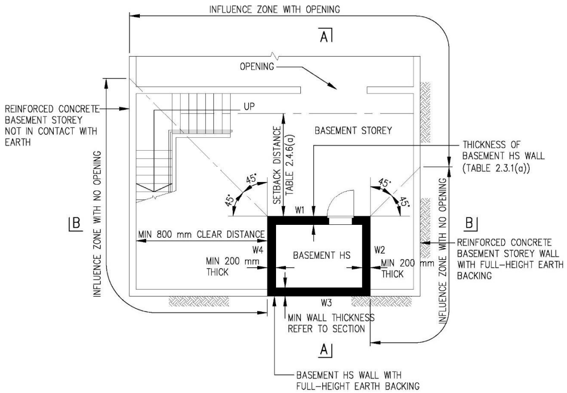
FIGURE 2.4.6(a) PLAN OF A BASEMENT HS
