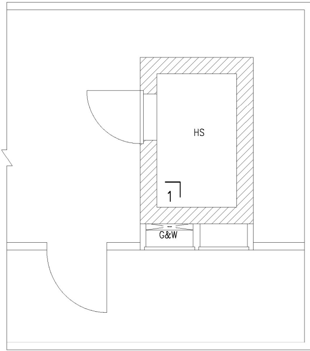
TYPICAL SHELTER PART PLAN OF GAS AND WATER OPENING WITHOUT ELBOW (TYPE B)
