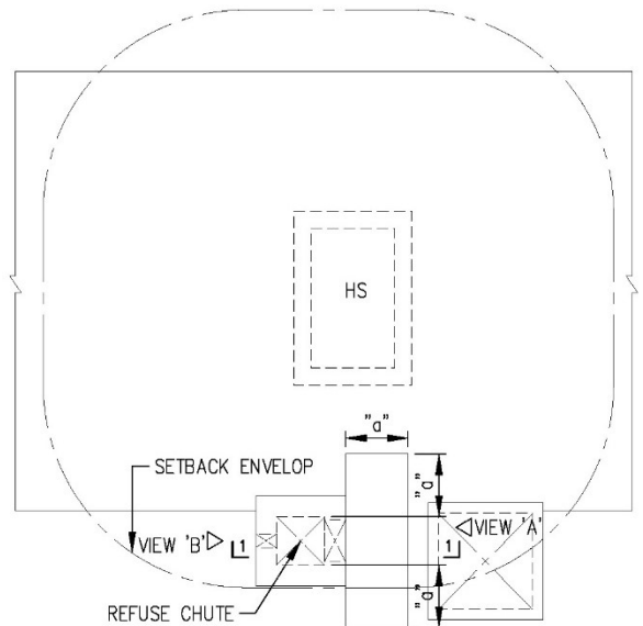
TYPICAL SHELTER ROOF PART PLAN WITH REFUSE CHUTE WITHIN SETBACK ENVELOPE HS
